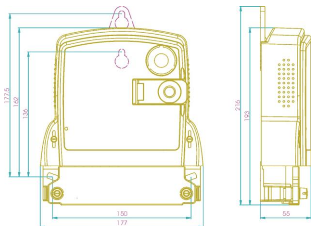
Fig. 6 – Meter with a short terminal cover and an additional top meter fixing element
