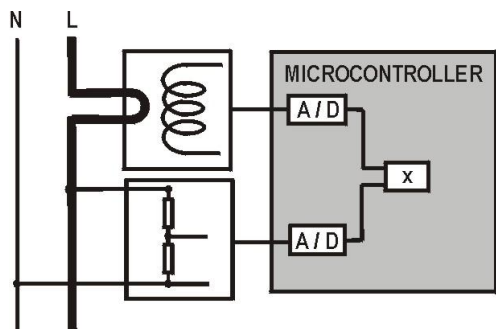
Fig. 8: Metering element
