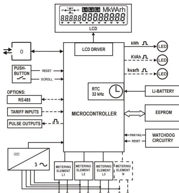
Fig. 7: Meter block-diagram
