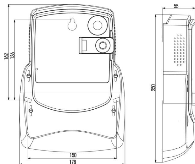
Fig. 5 – Meter with a long terminal cover
