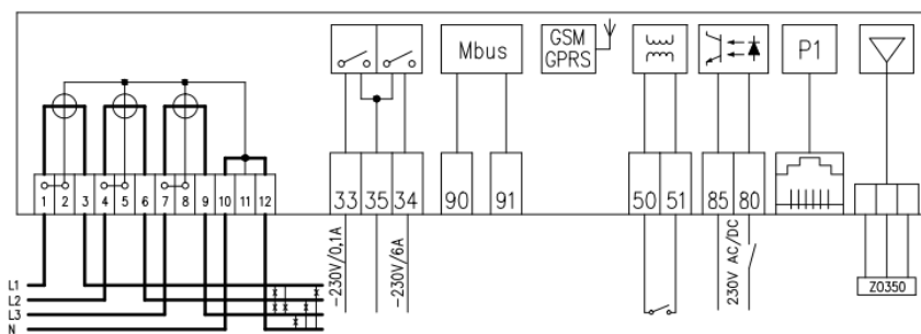
Figure 8: MT382 meter connection diagram – direct connection
